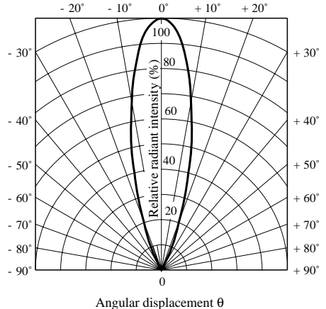
Fig. 11-b Radiation Diagram (GL561)
